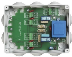
306-0007 2-relay box with PSU
