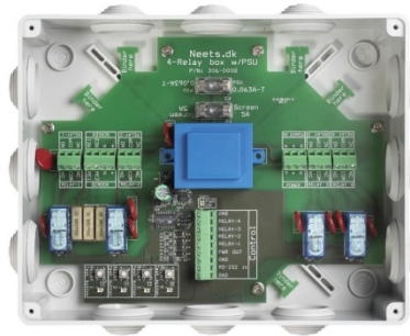
306-0008 4-relay box with PSU
